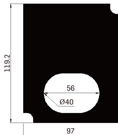
Fig.10c(unit: mm)
